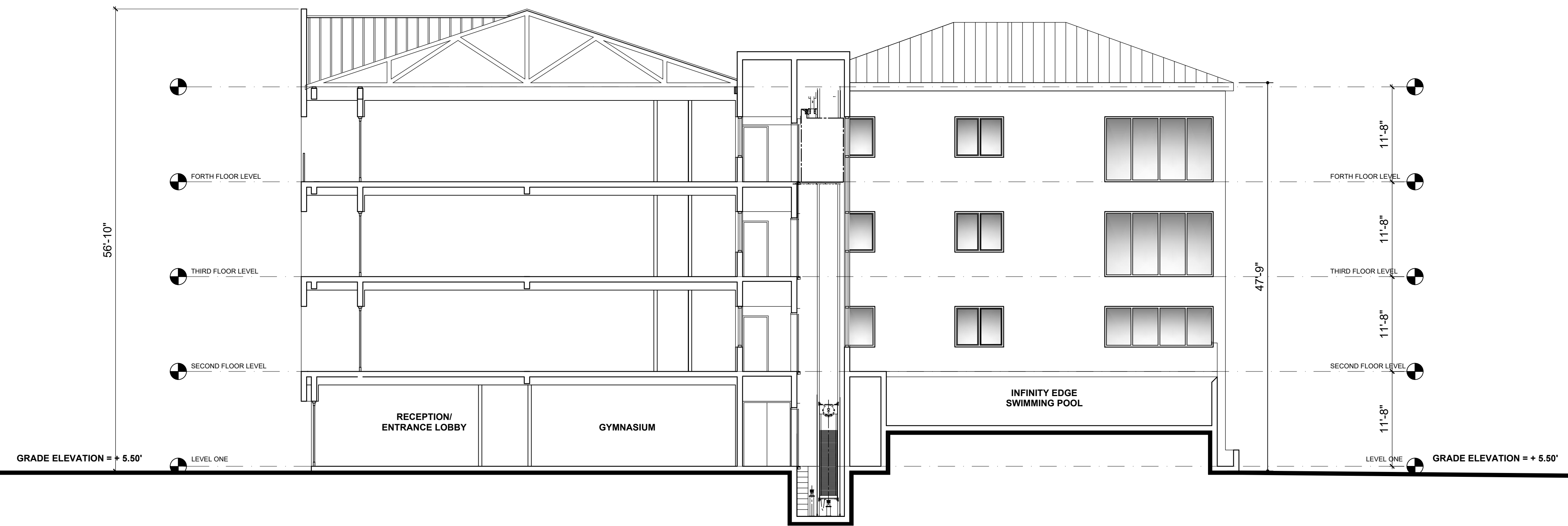
SECTION A - A
